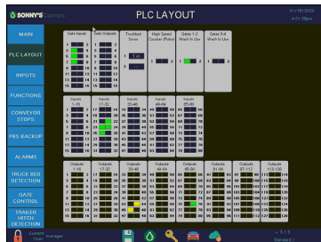
Graphic representation of the i/o modules inside
