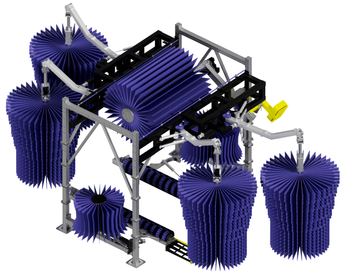
Compact Top Brush With DoubleJog Entrance and Exit Wraps and Tire Brush with SFTBG18 Rocker Brush. Shown with Optional Powder Coating
