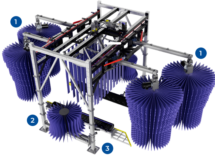
SFM901 Mitter with Straight Entrance and Exit Wraps and Tire Brush with SFTBG18 Rocker Brush. Shown with Optional Powder Coating
