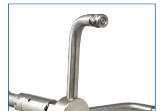
16 Zero-degree, 1/8in spray nozzles mounted on four swivel t-bars.
