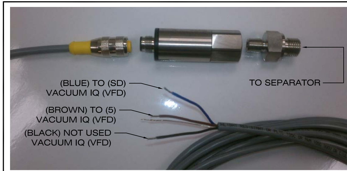
6 VACUUM IQ TO CABLE TO TRANSDUCER TO SEPARATOR
