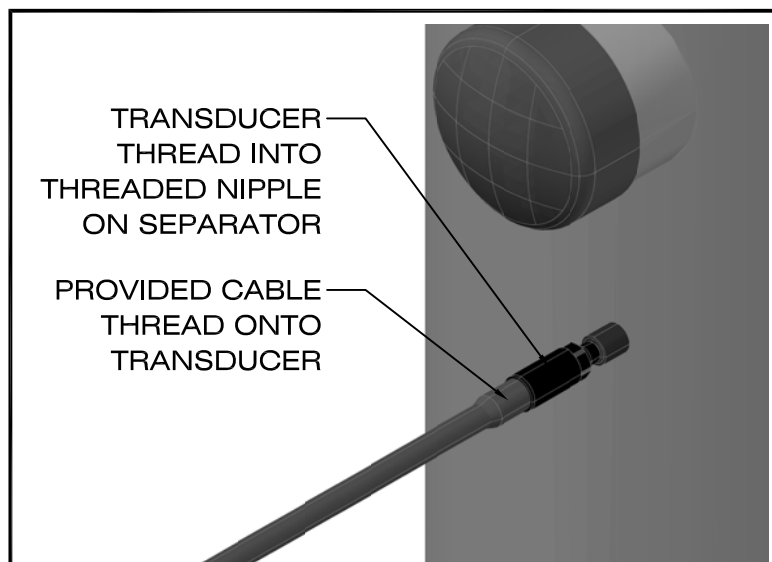
3 TRANSDUCER & CABLE TO SEPARATOR
