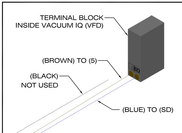
2 TRANSDUCER CABLE TO VACUUM IQ (VFD)
