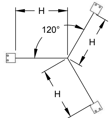
PLAN VIEW OF CONTACT SURFACES
