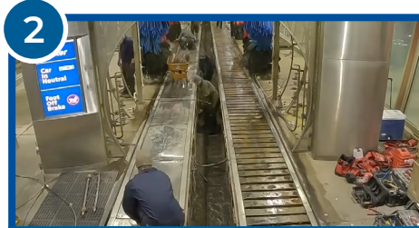
Removing Existing Conveyor Frames
